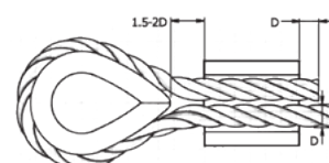
Before swaging
