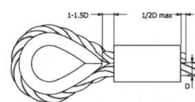
After swaging
