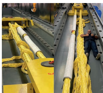
Fibre rope testing
